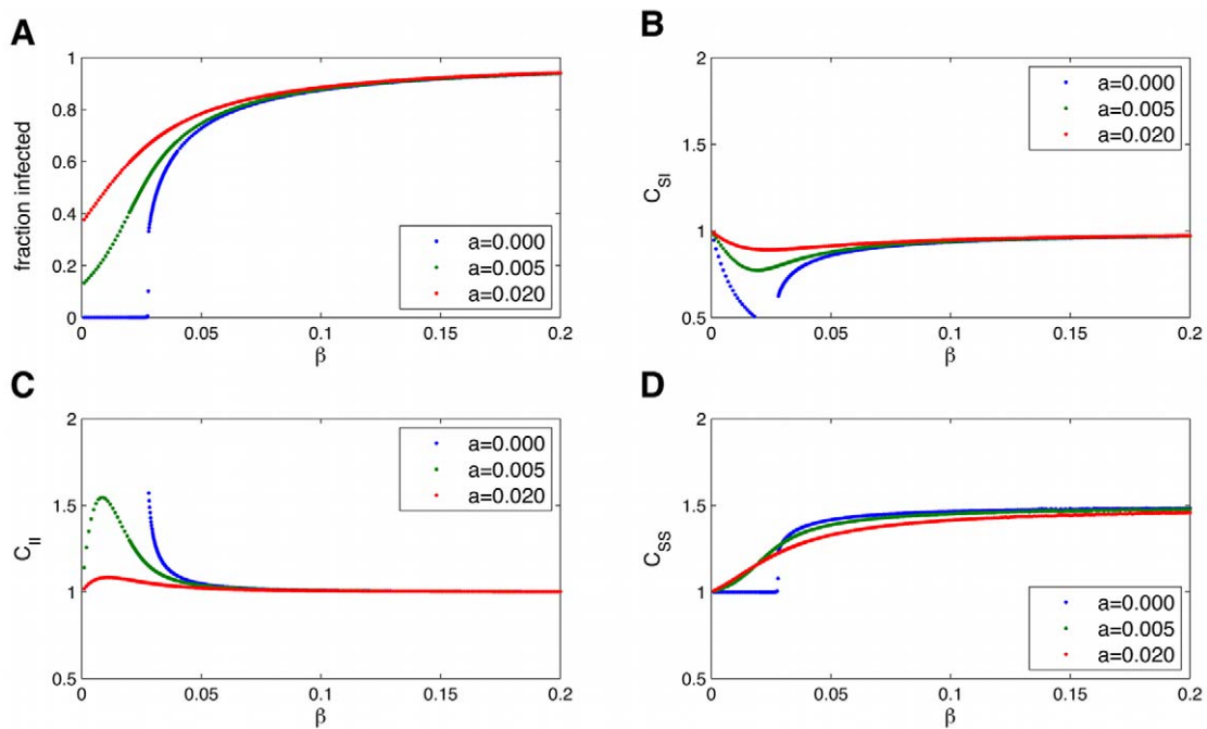
Figure 9. Dependence of the equilibrium fraction infected and correlations on the rate of transmission, \beta . Dependence of the equilibrium fraction infected (A) and correlations ( C_{SI} (B), C_{II} (C), C_{SS} (D)) on the rate of transmission, \beta . When a > 0 , expected in most social infections, there is no longer a threshold ( R_0 > 1 ) needed for the infection to invade the population. The network causes infected individuals to cluster C_{II} > 1 away from susceptible individuals C_{SI} < 1 , and this is more pronounced for larger \beta/a and lower fraction infected. Parameters are g = 0.035 , \phi = 0.64 , n = 3.0 .
