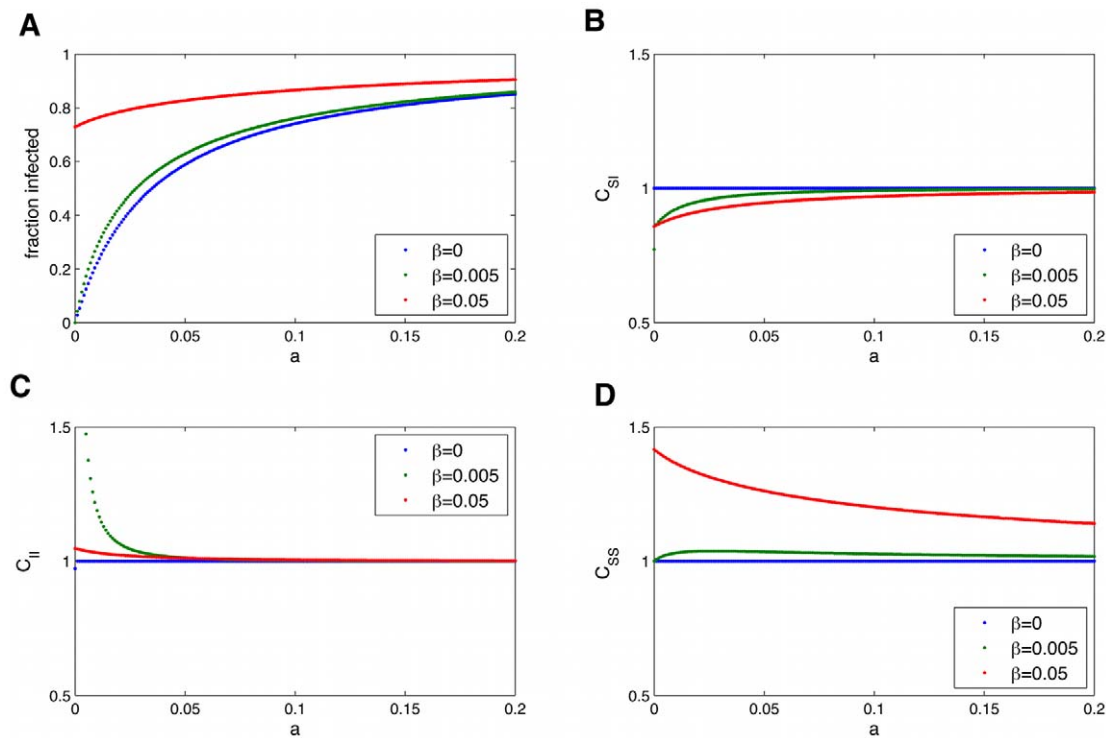
Figure 10. Dependence of the equilibrium fraction infected and correlations on the rate of automatic infection, a . Dependence of the equilibrium fraction infected (A) and correlations ( C_{SI} (B), C_{II} (C), C_{SS} (D)) on the rate of automatic infection, a . Parameters are g = 0.035 , \phi = 0.64 , n = 3.0 .
